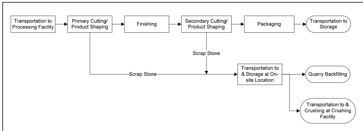
Figure 2. Process flow diagram for granite processing operations.
